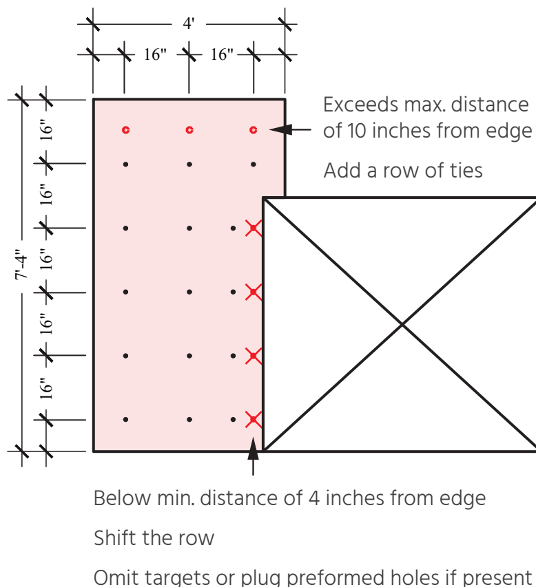
Figure 2 – Expanded example showing a sheet of rigid insulation that needs tie placement adjustments at the top and right side.
